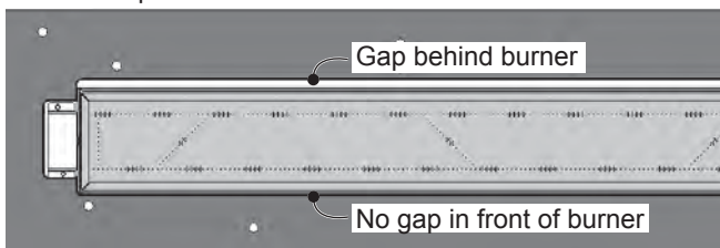
Top view—platform
